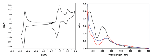
Fig. 3 (Left) Cyclic voltammogram of a 0.41 mM solution of \text{Ru}_2\text{Mn}-\text{OAc}_2 in 0.1 \text{ M } [n\text{Bu}_4\text{N}]\text{ClO}_4 in \text{CH}_3\text{CN} , at a scan rate of 50 \text{ mV s}^{-1} . (Right) UV-visible absorption spectra of a 0.41 mM solution of \text{Ru}_2\text{Mn}-\text{OAc}_2 in 0.1 \text{ M } [n\text{Bu}_4\text{N}]\text{ClO}_4 in \text{CH}_3\text{CN} , in oxidation states, (black) \text{Ru}_2(\text{II})\text{Mn}(\text{II}) , (red) \text{Ru}_2(\text{III})\text{Mn}(\text{II}) and (blue) \text{Ru}_2(\text{II})\text{Mn}(\text{III}) .
