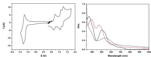
Fig. 2 (Left) Cyclic voltammogram of a 0.25 mM solution of \text{Ru}_2\text{Co}-\text{OAc}_2 in 0.1 \text{ M } [n\text{Bu}_4\text{N}]\text{ClO}_4 in \text{CH}_3\text{CN} , at a scan rate of 100 \text{ mV s}^{-1} . (Right) UV-visible absorption spectra of a 0.25 mM solution of \text{Ru}_2\text{Co}-\text{OAc}_2 in 0.1 \text{ M } [n\text{Bu}_4\text{N}]\text{ClO}_4 in \text{CH}_3\text{CN} , in oxidation states (black) \text{Ru}_2(\text{II})\text{Co}(\text{II}) , (red) \text{Ru}_2(\text{II})\text{Co}(\text{III}) and (blue) \text{Ru}_2(\text{III})\text{Co}(\text{III}) .
