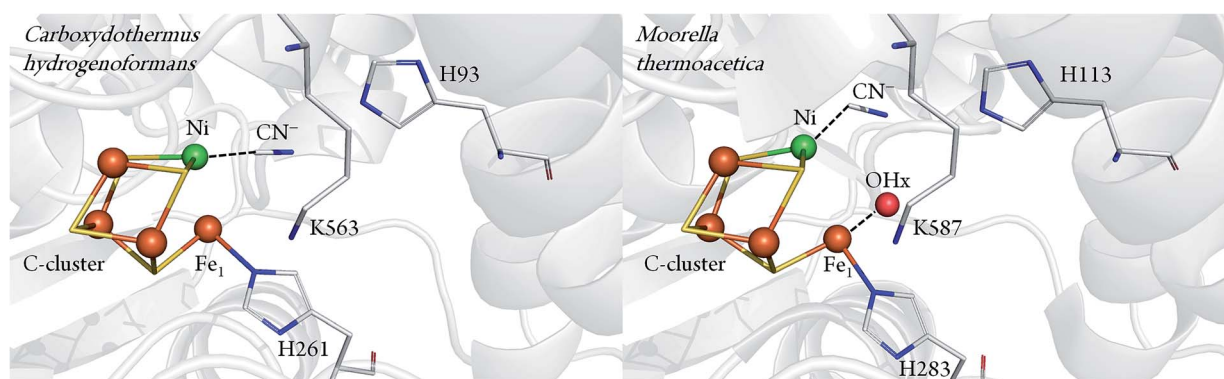
Fig. 1 Comparison between CN - bound C-cluster of CODHII Ch (pdb 3I39) and CODH Me (pdb 3I04), according to ref. 7 and 8.
