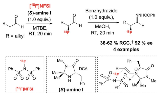
Scheme 5 Chiral imidazolidinone ( S )-I for the enantioselective ^{18}\text{F} -fluorination of aldehydes with [ ^{18}\text{F} ]NFSI. \dagger RCC determined by radio-HPLC relative to [ ^{18}\text{F} ]NFSI. DCA = dichloroacetic acid. For [ ^{18}\text{F} ]NFSI, SA = 0.05 \mu\text{mol}^{-1} , ( n = 3 ).
