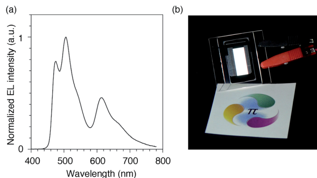
Fig. 9 White OLED with a single-layer architecture. (a) An electroluminescence spectrum at a current density of 0.1 mA cm ^{-2} . (b) A picture of the device with an emitting area of 16.6 mm \times 6 mm. The sheet under the device is showing a color reference printed on white paper, and the original colors can be found at http://www.jst.go.jp/erato/isobe/ .
