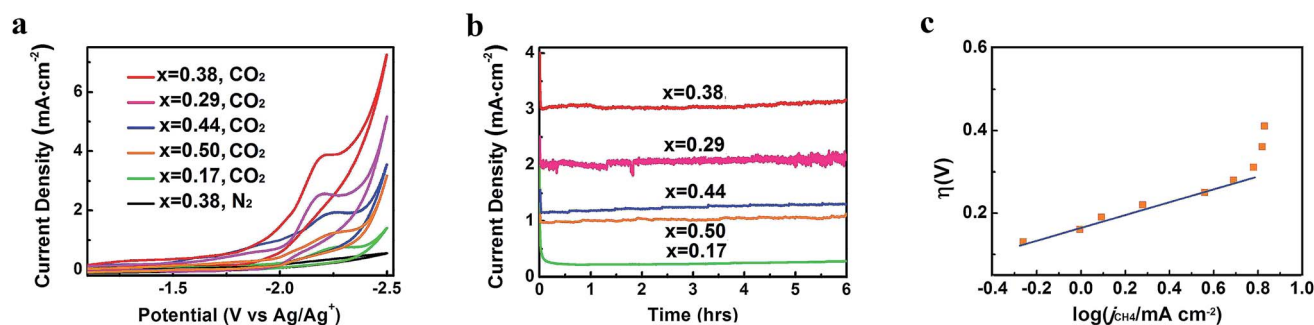
Fig. 4 CO 2 reduction performance of Zn-MOF/CP cathodes. (a) CV traces. (b) Current density profiles. (c) Tafel plot for CH 4 of the Zn-MOF/CP cathode using Zn-MOF synthesized at x = 0.38 .
