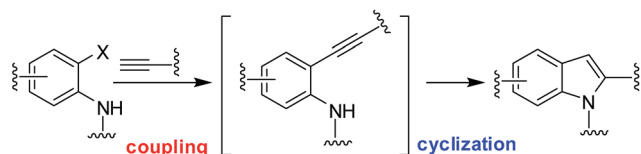
Scheme 1 Synthesis of indoles via the one-pot coupling-cyclization strategy.
