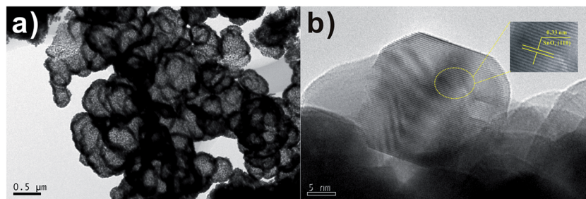
Fig. 4 (a) TEM (b) HRTEM images of SnO 2 samples after calcination at 550 °C for 3 h with 1 : 2 molar ratio of D-glucose and SnCl 2 ·2H 2 O.
