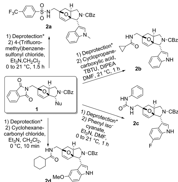
Fig. 3 Examples of functionalized compounds 2 after the first step. * Deprotection condition: hydrazine, 2 M HCl (aq.), MeOH, 21 °C, 1 h.
