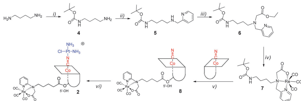
Scheme 1 Synthesis scheme towards [{Re}- cis -PtCl(NH 3 ) 2 ] + (2): (i) Boc 2 O; (ii) py-2-CHO, NaBH 4 ; (iii) BrCH 2 CO 2 Et; (iv) [NEt 4 ] 2 [ReBr 3 (CO) 3 ]; (v) TFA and then CDT, TEA; (vi) cisplatin, AgNO 3 .
