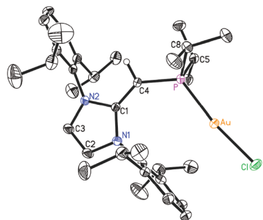
Fig. 7 Molecular structure of 8 with thermal ellipsoids at the 30% probability level. The hydrogen atom attached to C(4) is shown with an arbitrarily small thermal parameter; all other hydrogen atoms have been omitted for clarity. Selected bond lengths (Å) and angles (°): Au–P 2.2348(5), Au–Cl 2.2991(5), P–C(4) 1.7442(19), C(1)–C(4) 1.376(3), P–C(5) 1.848(2), P–C(8) 1.845(2), P–Au–Cl 171.40(2), C(4)–P–Au 122.82(7), P–C(4)–C(1) 136.20(15), C(4)–P–C(5) 105.69(10), C(4)–P–C(8) 104.31(10), Au–P–C(5) 106.89(7), Au–P–C(8) 110.83(7).
