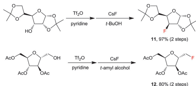
Scheme 7 Selected examples for the preparation of fluorinated bio-active molecules by fluorination with CsF in a t -alcohol solvent.
