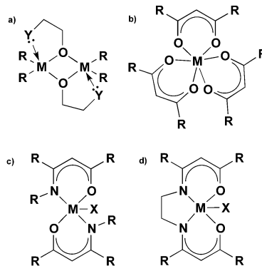
Fig. 17 Single-source precursors for gallium and indium oxide ( M = \text{Ga, In} ).
