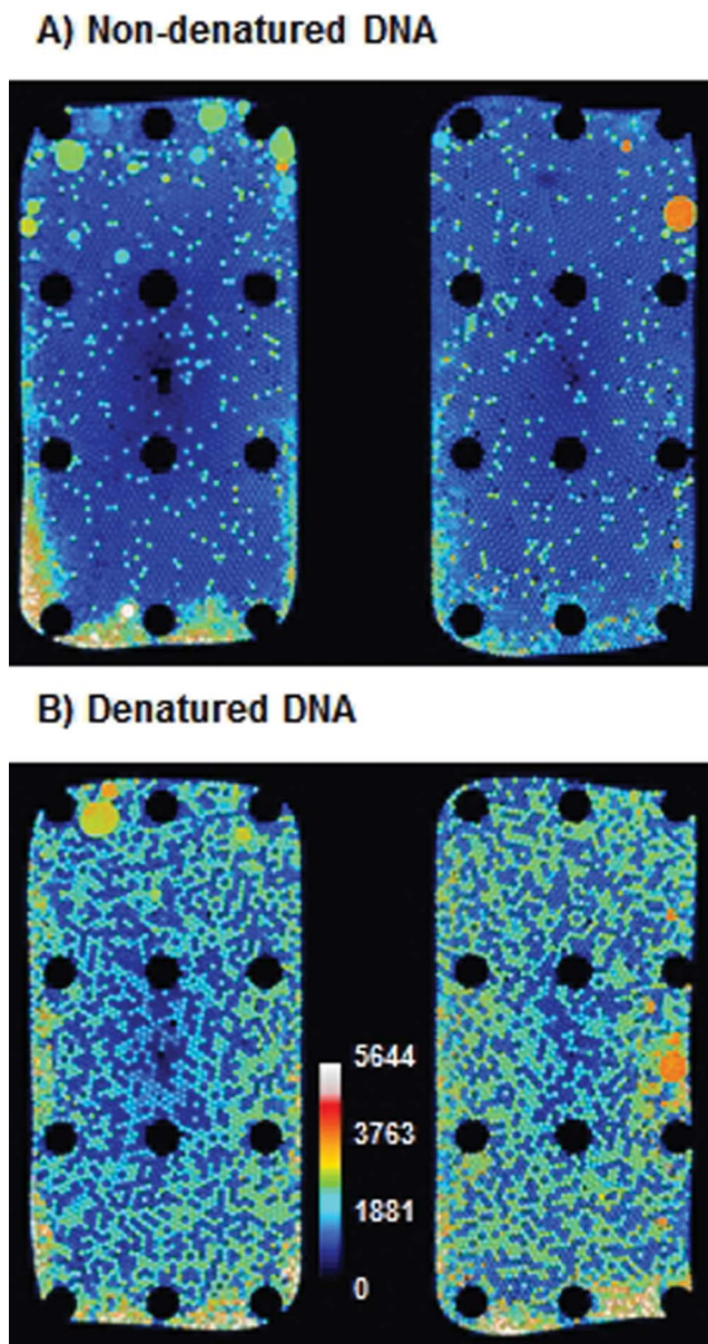
Fig. 3 False color fluorescence image of ddLAMP without (A) and with (B) heat denaturation of DNA prior to emulsification. In (B), an ~6-fold increase in droplets with a positive fluorescence signal compared to (A) can be observed (10.4% positive droplets in (A) compared to 58.0% positive droplets in (B)). As explained above some droplets have merged or have evaporated partially (e.g. A) in the lower left edge). These were excluded from the analysis. The increase in fluorescence on the edge might originate from increasing salt concentrations as the droplets partially evaporate. The increasing salt concentrations might lead to an unspecific quenching of the fluorescence.
