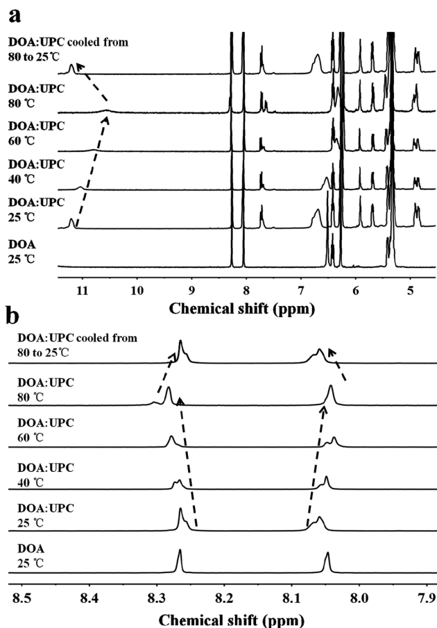
Fig. 2 Variable-temperature ^1\text{H} NMR spectra of DOA and DOA : UPC. (a) ^1\text{H} NMR spectrum of DOA at 25 °C (bottom) and ^1\text{H} NMR spectra of DOA : UPC at 25, 40, 60, 80 °C and cooled from 80 to 25 °C in the 4.5–11.5 ppm region. The arrow represents the changing trend of uracil NH chemical shift. (b) ^1\text{H} NMR spectrum of DOA at 25 °C (bottom) and ^1\text{H} NMR spectra of DOA : UPC at 25, 40, 60, 80 and cooled from 80 to 25 °C in the 7.9–8.5 ppm region. The arrows represent the changing trend of adenine CH chemical shifts. The mixing ratio (DOA : UPC) was 1 : 1. The sample was allowed to equilibrate for 5 min at each temperature (1,1,2,2-tetrachloroethane- d_2 -dimethyl sulfoxide- d_6 , 4 : 1).
