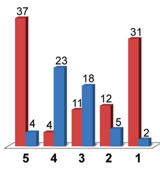
Fig. 7 Faradic yields (in %) for CO (red) and H 2 (blue) during the bulk electrolysis of 1 mM solutions of compounds 1–5 under CO 2 in DMF/H 2 O (95 : 5), TBAPF 6 0.1 M with an applied current of 300 μA during 4 h.
