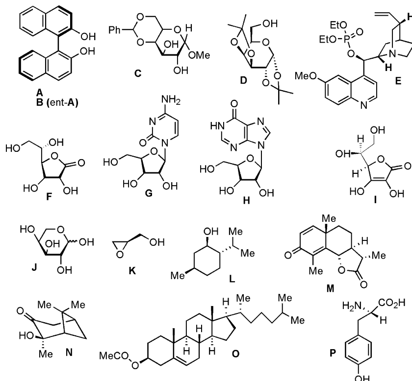
Fig. 1 Chiral ligands used in nitrile oxides 1,3-dipolar cycloaddition reactions.
