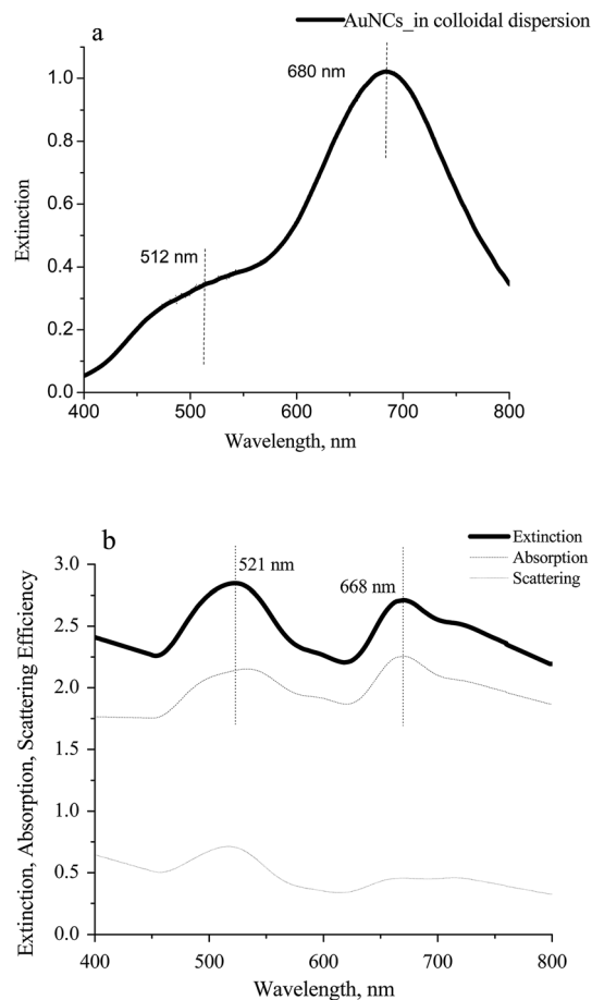
Fig. 3 Normalized UV-vis spectra of the Ag@AuNCs in aqueous dispersion of 250 fM (a). The DDA simulation of extinction, absorption and scattering efficiency spectra of hollow bimetallic Ag@Au nano-cage (b).
