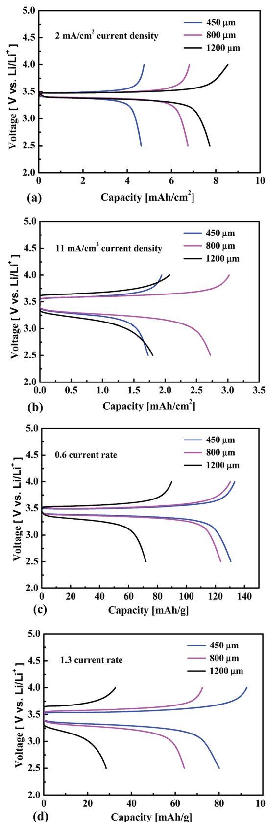
Fig. 3 Comparison of the charge-discharge curves at 2 \text{ mA cm}^{-2} (a), 11 \text{ mA cm}^{-2} (b), 0.6 C-rate (c) and 1.3 C-rate (d) for the cells using different cell size of metal foams.
