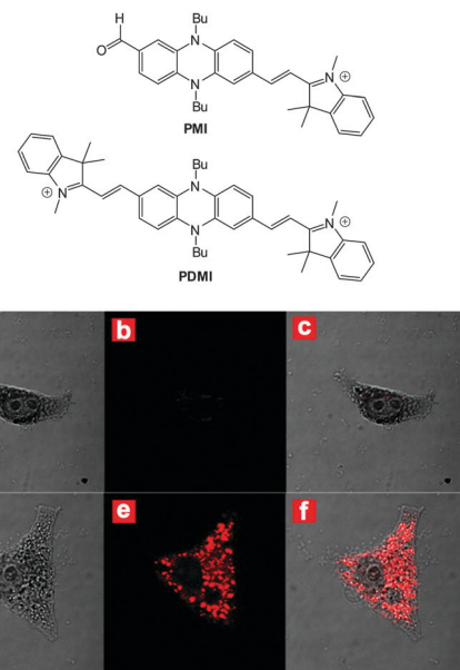
Fig. 32 Top: structures of PMI and PDMI . Bottom: images of HeLa cells incubated with PMI : bright-field (a), dark-field (b) and merged (c). Images of HeLa cells incubated with PMI then \text{CN}^- : bright-field (d), dark-field (e) and merged (f). Image reproduced with permission. 178
