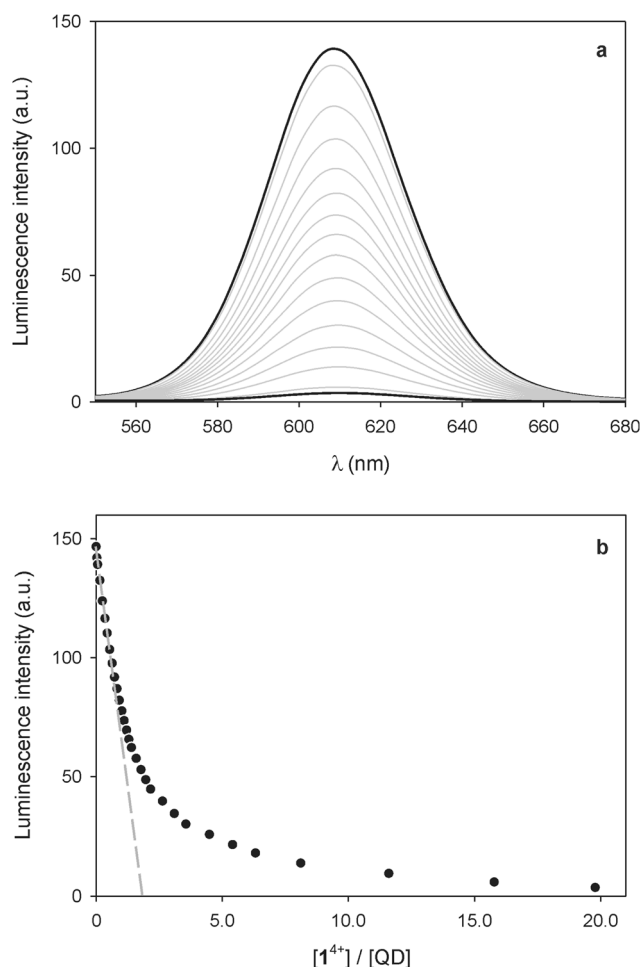
Fig. 3 (a) Luminescence spectral changes observed upon titration of 0.47 \mu\text{M} CdSe–ZnS QDs with 1 4+ . (b) Titration plot obtained from the QD luminescence intensity at 608 nm in the presence of increasing amounts of 1 4+ . The dashed line shows the tangent to the first part of the curve (it is a guide for the eye, not a fit). Conditions: air equilibrated CHCl 3 /CH 3 CN 9 : 1, room temperature, \lambda_{\text{exc}} = 500 nm.
