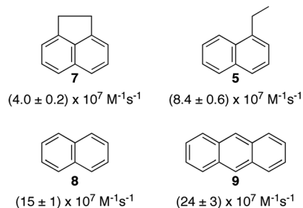
Scheme 6 Structure of guests that bind to the primary aggregates of sodium cholate and the quenching rate constants by iodide anions of the aggregate bound singlet excited states of the guests. The quenching rate constants correspond to average values in the presence of 20 and 40 mM sodium cholate. 31,32,35
