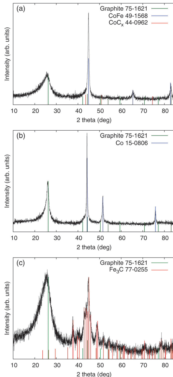
Fig. 2 XRD results of the (a) CoFe-CNfFs, (b) Co-CNfFs, and (c) Fe-CNfFs.
