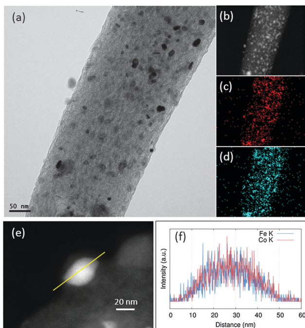
Fig. 1 (a) TEM image, (b) STEM image of the CoFe-CNfFs, EDS maps for (c) Fe and (d) Co, in the same STEM image. (e) Magnified STEM image and (f) linear EDS profile of the carbon layer enclosed metal particles with a roughly Co:Fe = 1:1 ratio.
