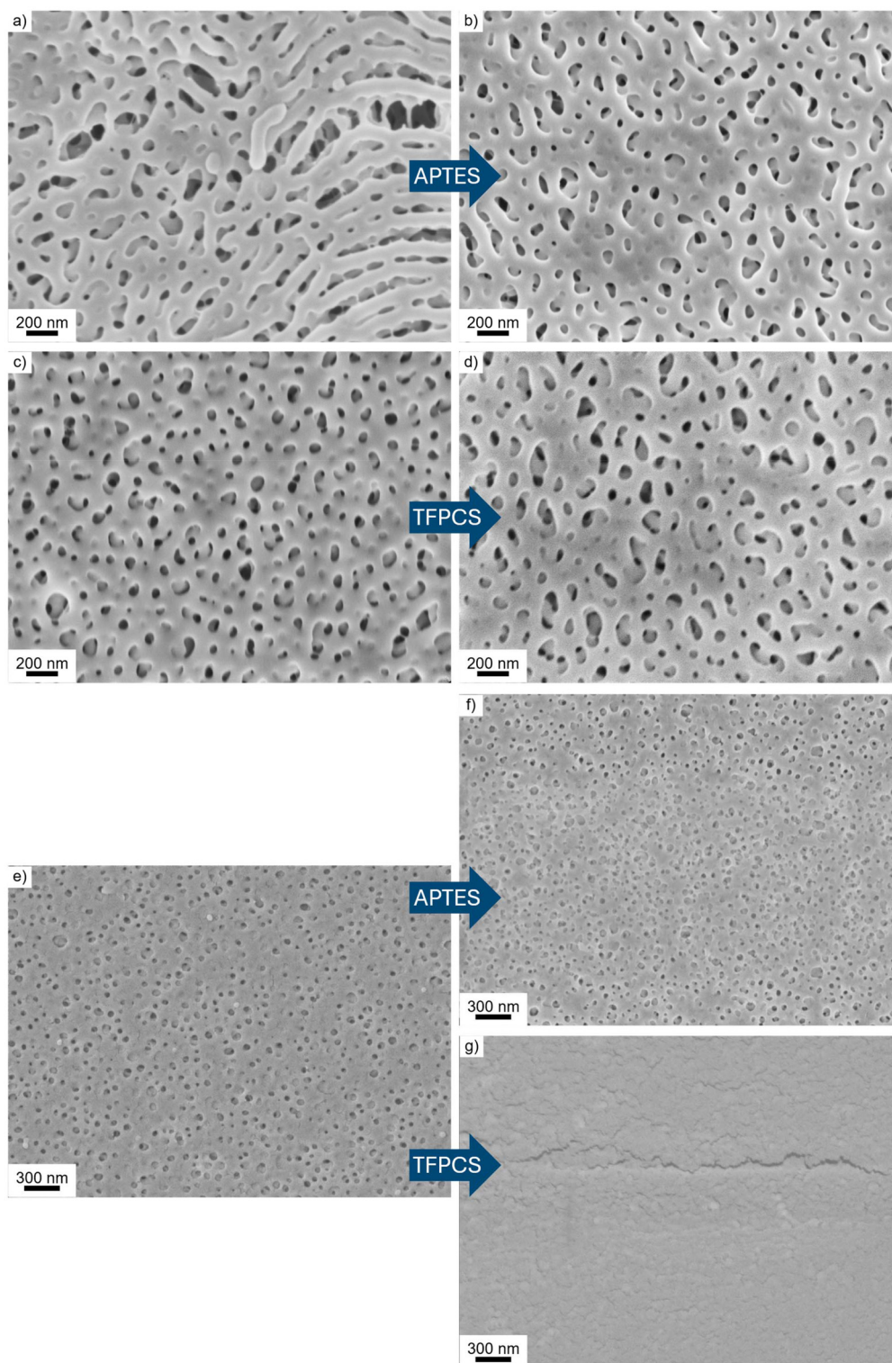
Fig. 5 Membranes based on the linear BCP are shown before post-modification (a, c) and after post-modification with APTES (b) and TFPCS (d). Membranes based on star-shaped BCPs ( M3 ) before post-modification (e) and after post-modification with APTES (f) and TFPCS (g).
