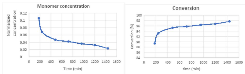
Fig. 4 Homopolymerization of P2VPS in a continuous flow reactor set-up: flow 0.2 \text{ ml min}^{-1} up to 1 \text{ ml min}^{-1} using a step of 0.1 \text{ ml min}^{-1} showed the correlation of monomer concentration and the conversion percentage in a quiescent experiment under ambient time and pressures.
