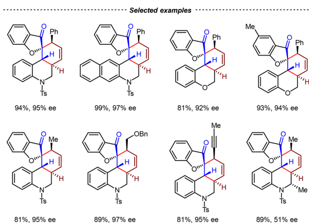
Scheme 43 Pd(0)-catalyzed tandem asymmetric Tsuji–Trost allylation and intramolecular [4+2] cycloaddition reactions.
