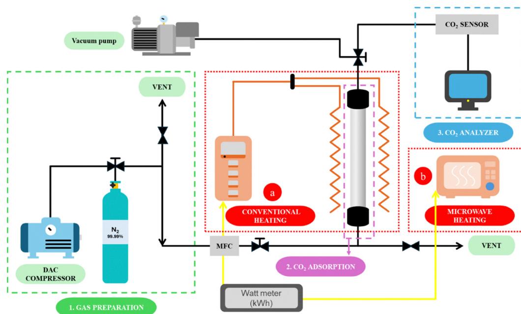
Fig. 23 Illustration of the direct air \text{CO}_2 capture process in a fixed-bed reactor: (a) regeneration through traditional thermal heating, and (b) regeneration utilizing microwave-assisted heating. Reproduced from ref. 173 with permission from Springer Nature, copyright 2025.
