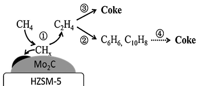
Fig. 12 Schematic diagram of coking pathways during CH 4 conversion over Mo 2 C/HZSM-5 catalyst. Reproduced from ref. 68 with permission from Elsevier, copyright 2014.
