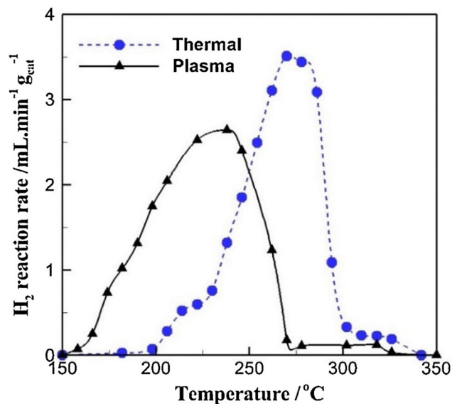
Fig. 22 \text{H}_2 temperature-programmed reduction (TPR) profiles comparing thermal and plasma-assisted reduction methods. Reproduced from ref. 168 with permission from John Wiley and Sons, copyright 2016.
