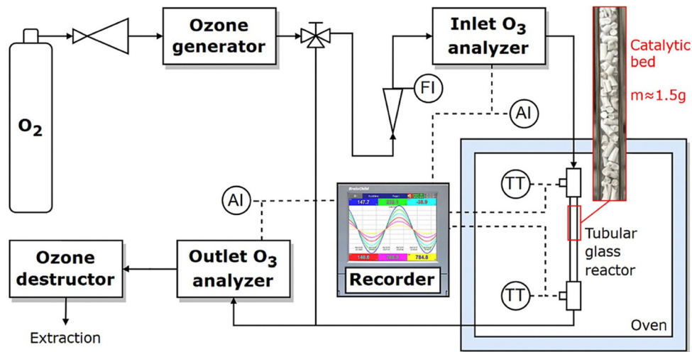
Fig. 19 Laboratory-scale setup for the regeneration of coked catalyst via ozonation as proposed by ref. 122. Reproduced from ref. 122 with permission from Elsevier, copyright 2023.
