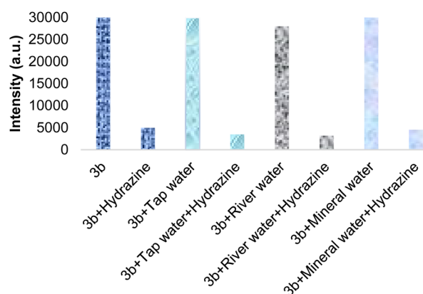
Fig. 7 Emission intensity of SBC 3b (0.5 \mu M; 537 nm) after the addition of different water samples in methanol with and without hydrazine.
