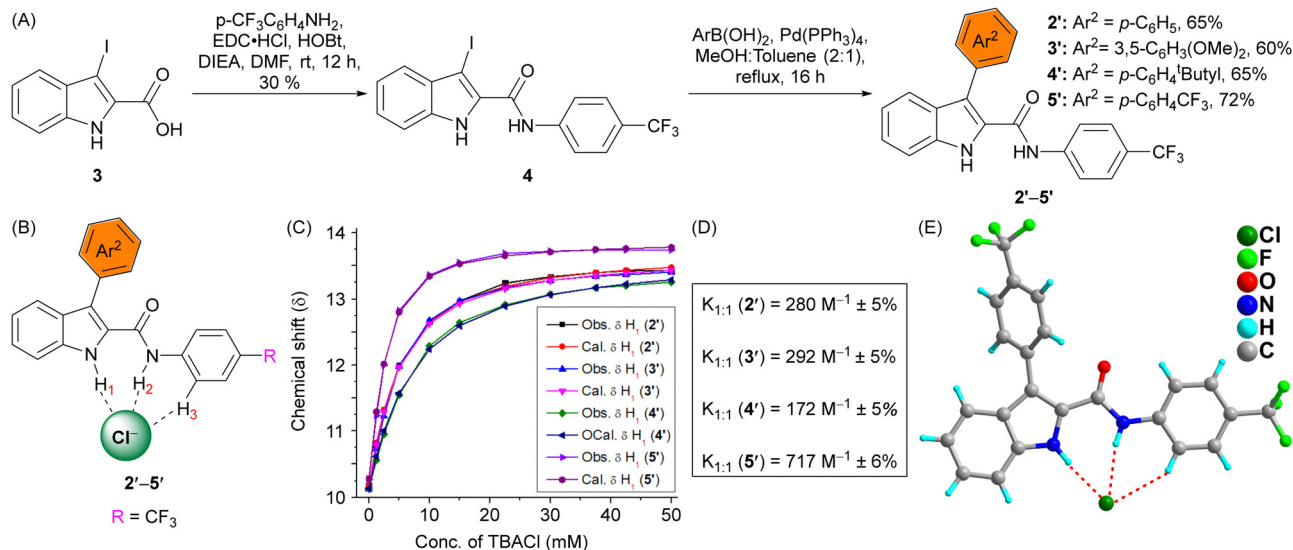
Fig. 2 Chemical synthesis of carriers 2'-5' (A). Chemical structure of the carriers showing binding interactions with the chloride anion (B). The plot of chemical shifts ( \delta ) of the \text{H}_1 proton vs. concentrations of TBACl added, fitted to a 1:1 binding model of BindFit for the active carriers 2'-5' (C). Binding constant values of carriers 2'-5' (D). (E) X-ray crystallographic structure of 5' with the chloride anion (D).
