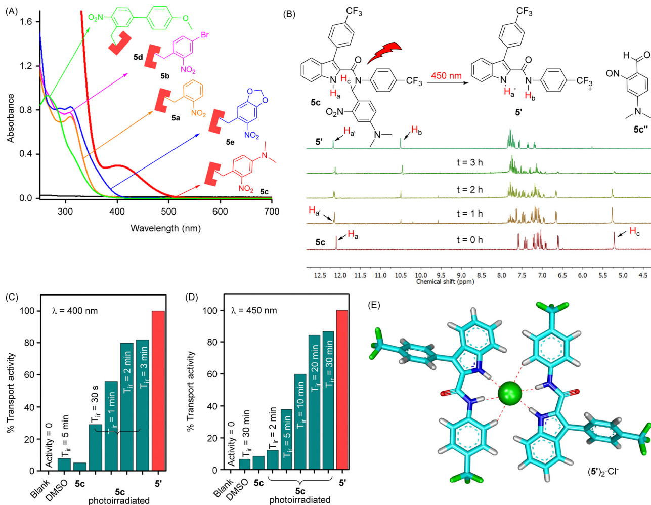
Fig. 6 UV-visible absorption spectrum of o -NB protected procarrier compounds 5a–5e (A). Phototriggered release of an active carrier 5' from ONB-protected procarrier 5c monitored by 1 H NMR studies recorded in DMSO- d 6 photoirradiated using 450 nm LEDs at different intervals of time (B). Normalized ion transport activity data of 5c upon photoirradiation at 400 nm (C), and 450 nm (D), respectively. The geometry-optimized structure of the [( 5' ) 2 + Cl - ] complex (E).
