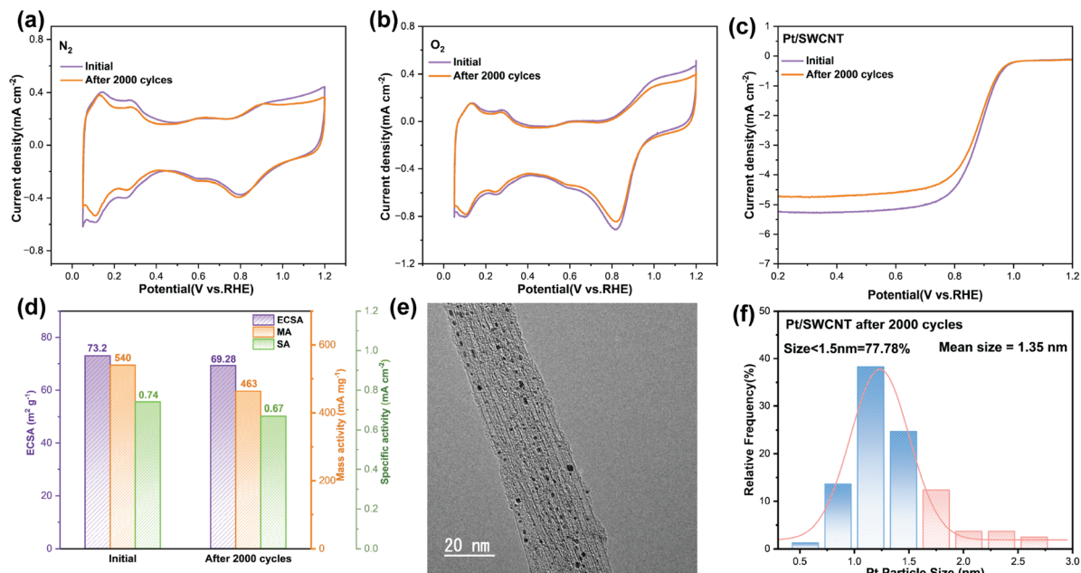
Fig. 7 Electrochemical and structural characterization of Pt/SWCNT catalysts before and after accelerated stress testing (AST). (a and b) CV curves in N_2 - (a) and O_2 -saturated (b) 0.1 M HClO_4 at a scan rate of 50\text{ mV s}^{-1} . (c) LSV curves under O_2 -saturated 0.1 M HClO_4 at a rotation rate of 1600 rpm. (d) Electrochemically derived ECSA, MA and SA values before and after AST. (e) TEM image of the Pt/SWCNT catalyst after AST. (f) Particle size distribution histogram of Pt nanoparticles after AST.
