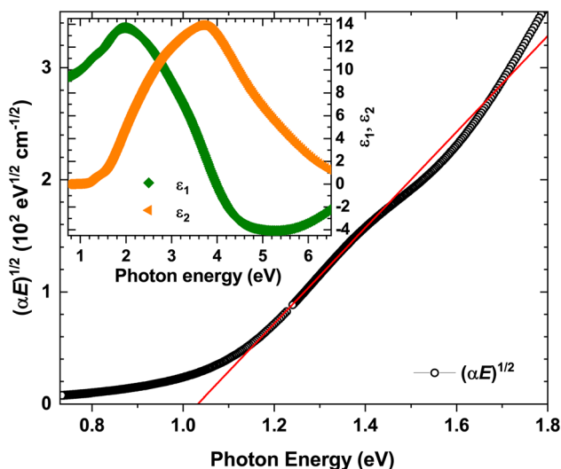
Fig. 11 Tauc plot for indirect optical transitions [ (\alpha E)^{1/2} ] and band-gap determination by linear projection to zero absorption (red line). Inset: real ( \epsilon_1 ) and imaginary ( \epsilon_2 ) parts of the dielectric function.
