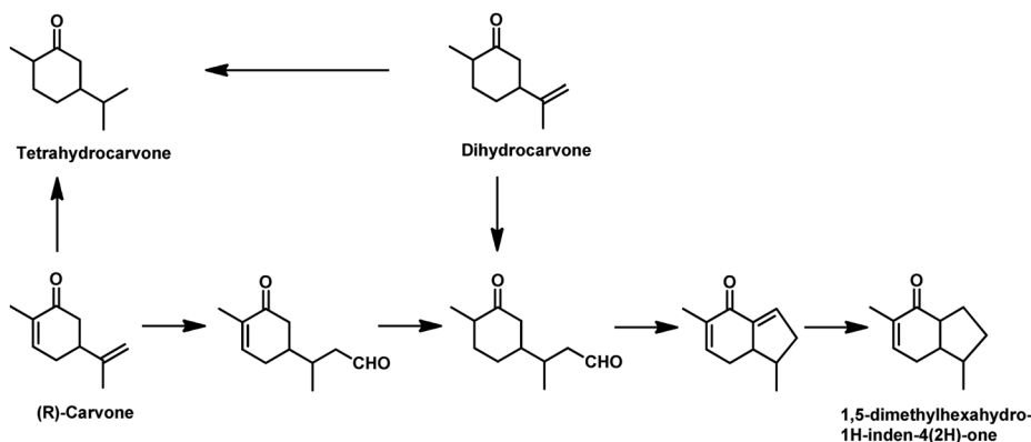
Scheme 26 Synthesis of 1,5-dimethylhexahydro-1 H -inden-4(2 H )-one from ( R )-carvone. Reaction conditions: Rh(CO) 2 (acac), dppp, PPTS, CO/H 2 (1 : 1, 650 psi), toluene, 120 °C, 22 h.
