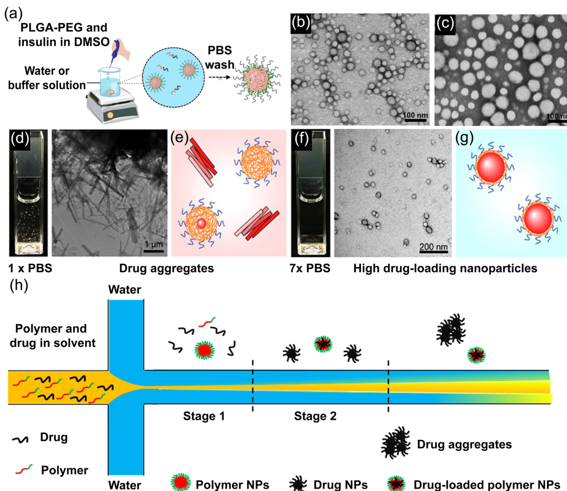
Fig. 6 Nanoprecipitation for fabrication of nanocarriers of pharmaceutical active ingredients. (a) Schematic representation of the preparation of the insulin-loaded PNPs (Ins-NPs) and (c) PLGA-PEG NPs without insulin. 131 (d) The snapshot of the mixtures, TEM images, and schematic for the nanoparticles produced by (d) and (e) bad salt concentration and (f) and (g) good salt concentration in producing 50 wt% docetaxel-loaded PLGA10k-PEG5k nanoparticles. 128 (h) Schematic representation of the formation of the polymer-stabilized peroxide antimalarial drug nanoparticle and the drug release profile of the nanoparticle and unencapsulated powder in the bio media. 81
