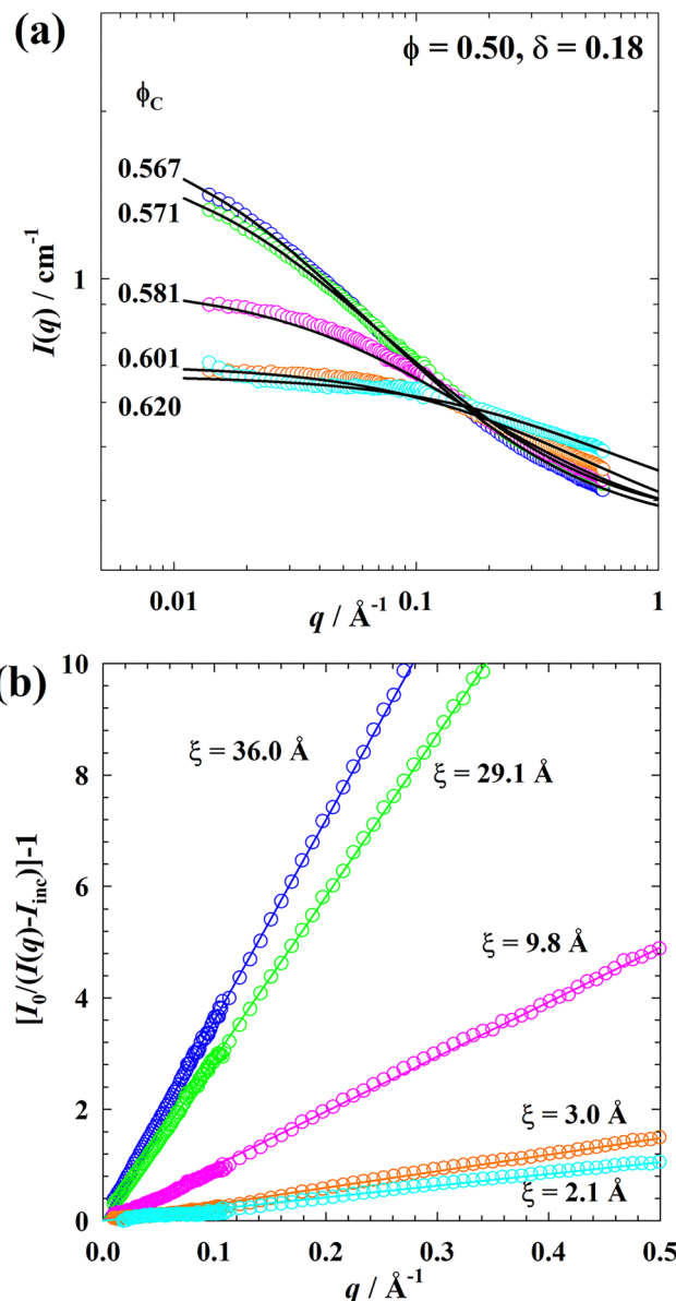
Fig. 4 (a) C-contrast SANS curves plotted on a double logarithmic scale and (b) [I_0/(I(q) - I_{inc})] - 1 plotted versus q for the quasi-ternary system D 2 O–cyclohexane–D 12 /cyclohexane (85/15)–2-propanol-OD/1-propanol-OD measured as a function of the total alcohol volume fraction \phi_C at \delta = 0.18 , \phi = 0.50 , and T = 25.0 °C. \xi -Values were obtained from the slope of the plot.
