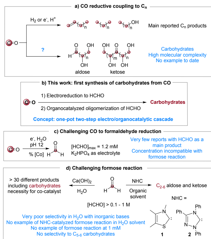
Scheme 1. a) CO conversion to C n compounds; b) Overview of the present work; c) Status and challenges of CO to HCHO electro-conversion; d) Status and challenges of formose reaction catalyzed by inorganic base (in H 2 O) and by NHC (in organic solvent).
