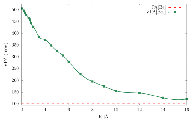
Fig. 2 Be_2 vertical positron affinity at the DMC level (in green line). The dashed line indicate the Be atom positron affinity. Error bars represent one standard error on the mean.
