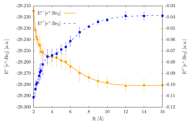
Fig. 3 Electronic energy ( E^e[e^+:Be_2] ), and positronic energy ( E^+ [e^+:Be_2] ) contributions. Error bars represent one standard error on the mean.
