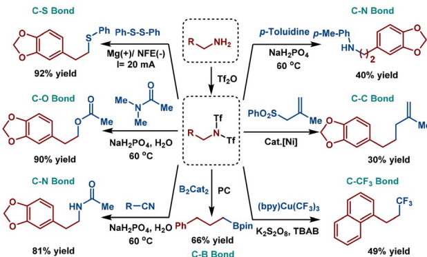
Scheme 25 Electrochemical C-B bond coupling of alkyl bistriflimides with B_2Cat_2 .
