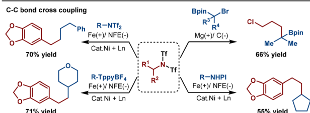
Scheme 23 Electrochemical C-C bond coupling of alkyl bistriflimides with aryl halides.
