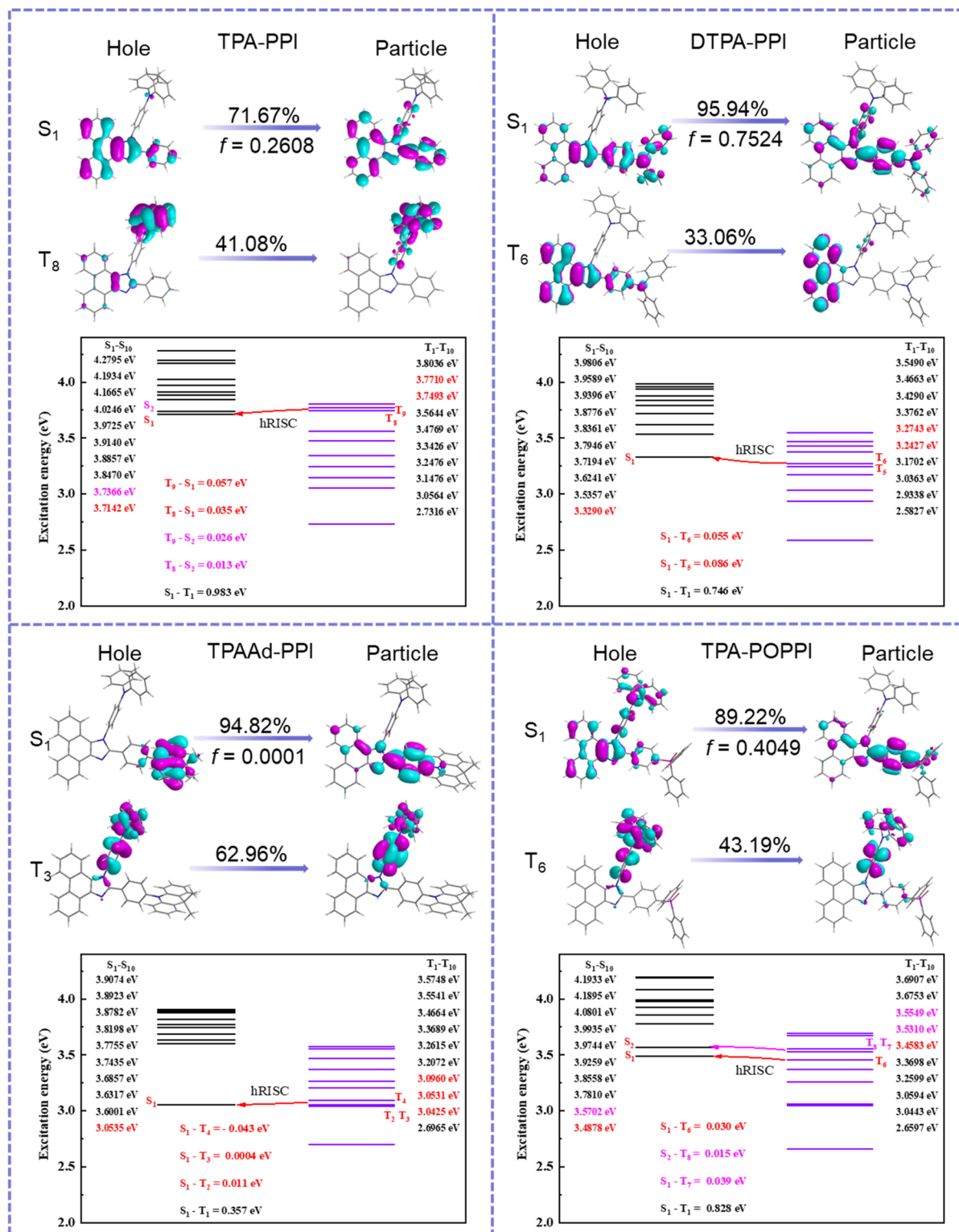
Fig. 3 The natural transition orbitals and the energy levels of the first ten singlet and triplet states of TPA-PPI, DTPA-PPI, TPAAd-PPI and TPA-POP.
