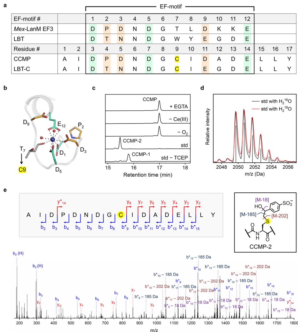
Fig. 2 Design of Ce(III)-binding peptides for site-specific oxidative thiol–ene coupling. (a) Amino acid sequences of Mex-LanM EF3, LBT, and CCMP mutants. EF-hand motifs are highlighted with a bold-bordered box. (b) A previously reported X-ray crystal structure of the 3rd EF-hand of Mex-LanM (PDB code: 8fns). Metal (Nd(III) in this case) and metal-bound water molecules are shown with blue and red spheres, respectively. (c) HPLC analysis of the reactions with 100 \mu M Ce(III)/CCMP and 10 mM 4VBS in 50 mM Tris–HCl, pH 7.4, followed by 1 mM TCEP treatment and the modified conditions. (d) Negative-ion mode MALDI-TOF/TOF analysis of CCMP-2 from the reactions with \text{H}_2^{16}\text{O} or \text{H}_2^{18}\text{O} . Vertical drop lines indicate the calculated isotope mass distribution of CCMP-2 [\text{M}-\text{H}]^- . (e) Tandem mass spectrometry fragmentation analysis of CCMP-2. Asterisks indicate the peptide fragments containing the modified cysteine.
