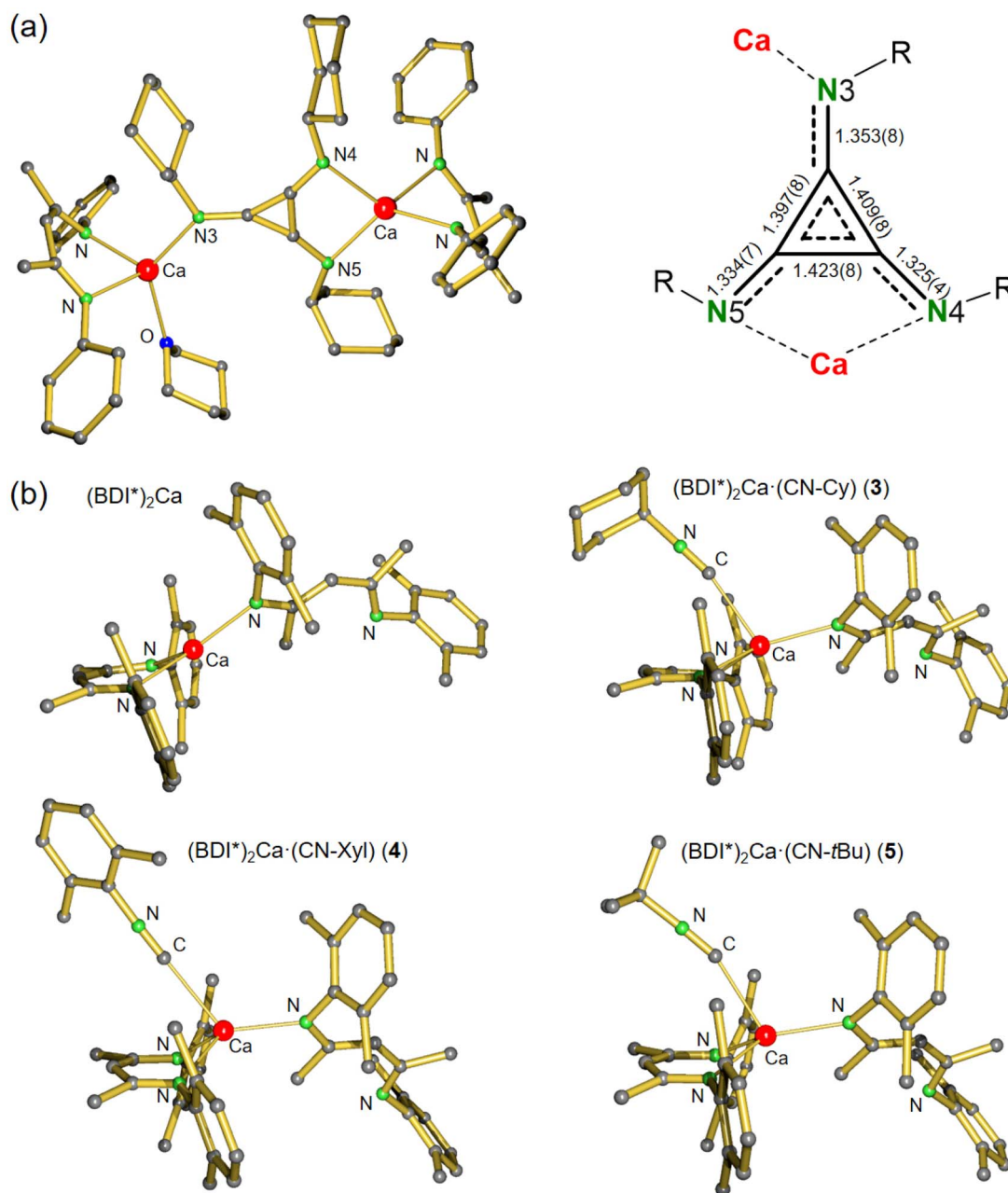
Fig. 2 (a) Crystal structure of [(\text{BDI}^*)\text{Ca}]_2(\text{C}_3(\text{NCy})_3)(\text{THP}) (2) and a detailed view of the triimino delatate dianion \text{C}_3(\text{NCy})_3^{2-} with bond distances in Å. H atoms and \text{Et}_2\text{CH} -groups have been omitted for clarity. (b) Comparison of the crystal structures of (\text{BDI}^*)_2\text{Ca}^0 with the isonitrile adducts 3 – 5 . H atoms and the \text{Et} groups of the \text{Et}_2\text{CH} substituents have been omitted for clarity.
