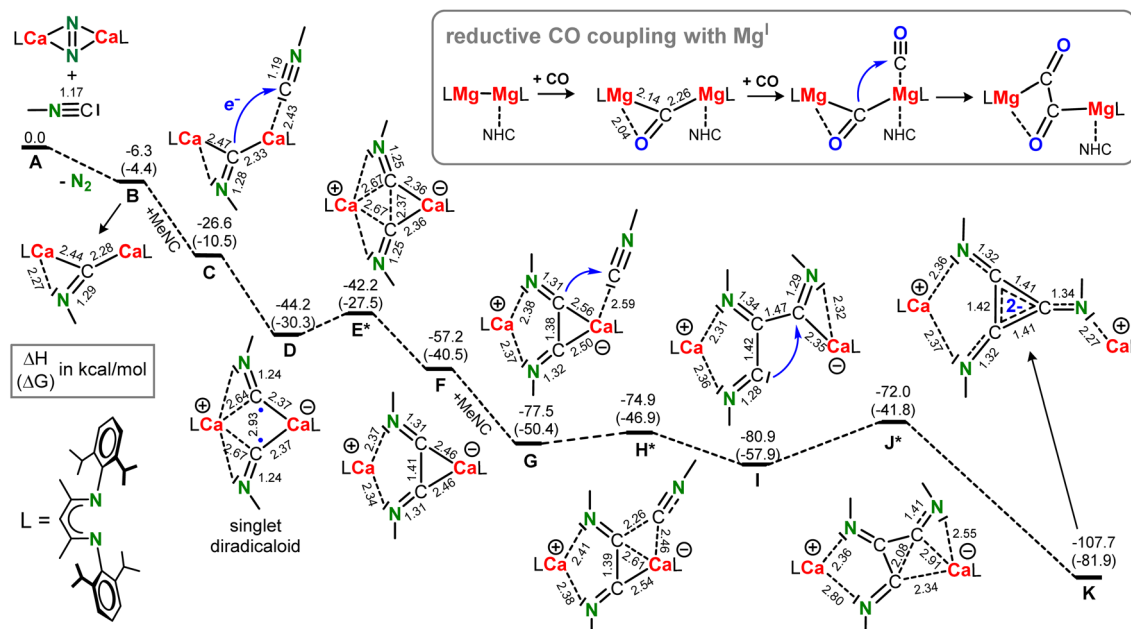
Scheme 4 Reductive coupling of isonitrile. Energy profile for triimino deltate formation calculated at the B3PW91-GD3BJ/def2tzvp//B3PW91-GD3BJ/def2svp level of theory for a model system with L = \text{DIPPBdi} and \text{MeN}\equiv\text{C} . \Delta H in \text{kcal mol}^{-1} . Between brackets: \Delta G (298 K) in \text{kcal mol}^{-1} . Selected bond lengths are given in Å. Inset: For comparison, reductive CO dimerization with (\text{DIPPBdi})\text{Mg-Mg}(\text{DIPPBdi}) activated with a N-heterocyclic carbene (NHC) follows a different pathway. 13
