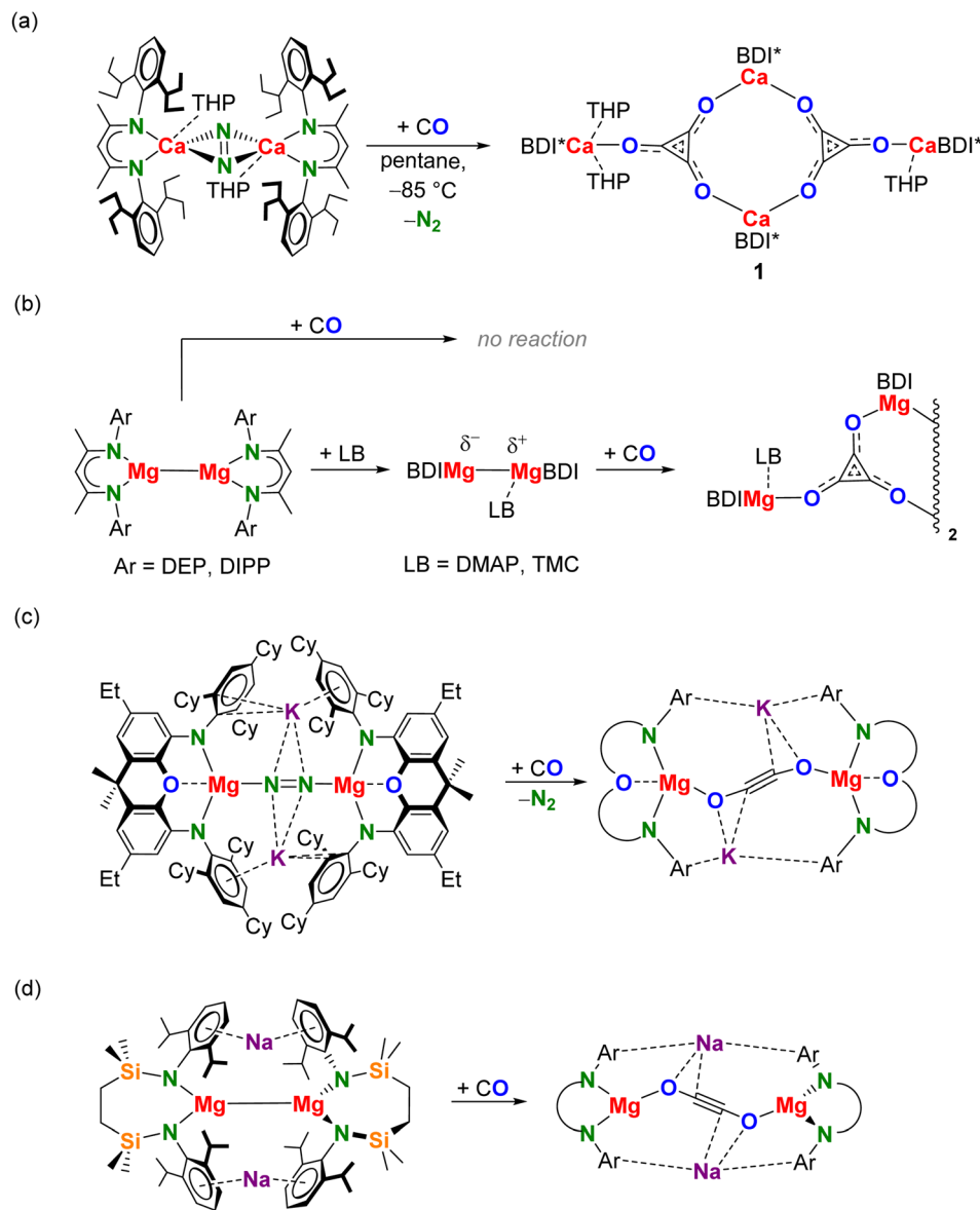
Scheme 2 (a) Reaction of [(\text{BDI}^*)\text{Ca}(\text{THP})]_2(\text{N}_2) with CO. (b) Reaction of \text{Mg}^{\text{I}} complexes with CO after prior polarization of Mg–Mg bond. 13,14 DEP = 2,6-Et-phenyl, DIPP = 2,6-iPr-phenyl, DMAP = 4-Me 2 N-pyridine, TMC = :\text{C}[\text{N}(\text{Me})\text{CMe}]_2 . (c) Reaction of a heterobimetallic Mg/K dinitrogen complex with CO. 18 (d) Reaction of a heterobimetallic Mg/Na complex with CO. 17
