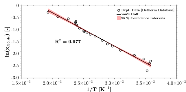
Fig. 6 Temperature-dependent KOAc solubility in HOAc (data: ref. 80).
