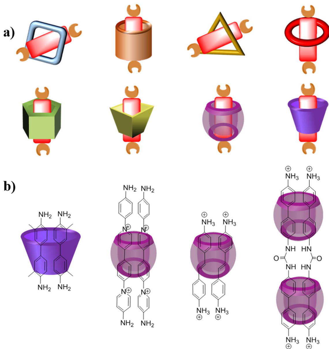
Fig. 1 Possible host-guest complex for the construction of COFRs (a) host-guest complex (1:1); (b) host-guest complex (1:2 and 2:2). Adapted from ref. 57 with permission from Royal Society of Chemistry, RSC Adv. , 2024, vol. 14, p. 30077-30083 Copyright 2024.
