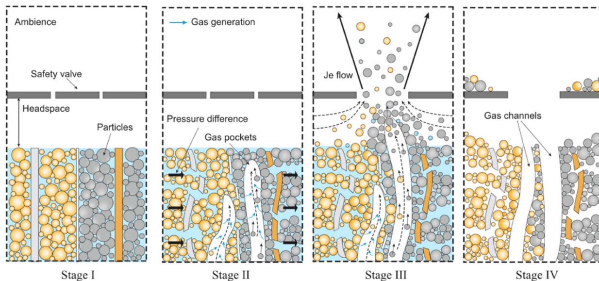
Fig. 13 (a) Diagram illustrating the mechanisms and change processes for the three main stages of thermal runaway, and (b) Particle release mechanism from a standard lithium-ion battery cell during thermal runaway. Figure has been reproduced from ref. 135 with permission from Elsevier, copyright 2023.
