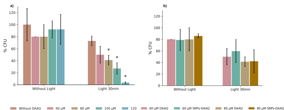
Fig. 8 (a) Inactivation of S. aureus ATCC 29213 mediated by DAAQ without light (left) and with blue LED (right) in PBS. DAAQ concentrations tested were 60 \mu M, 80 \mu M, 100 \mu M, and 120 \mu M. The bar graphs show the percentage of CFU mL -1 (average of triplicate experiments) surviving PDT, with respect to the initial inoculum that was not exposed to blue LED light and without DAAQ (control). (b) Comparative inactivation of S. aureus ATCC 29213 mediated by DAAQ 60 \mu M and 80 \mu M and SNPs-DAAQ 60 \mu M and 80 \mu M without light (left) and with blue LED (right) in PBS. The bars represented DSE- * p < 0.05 .
