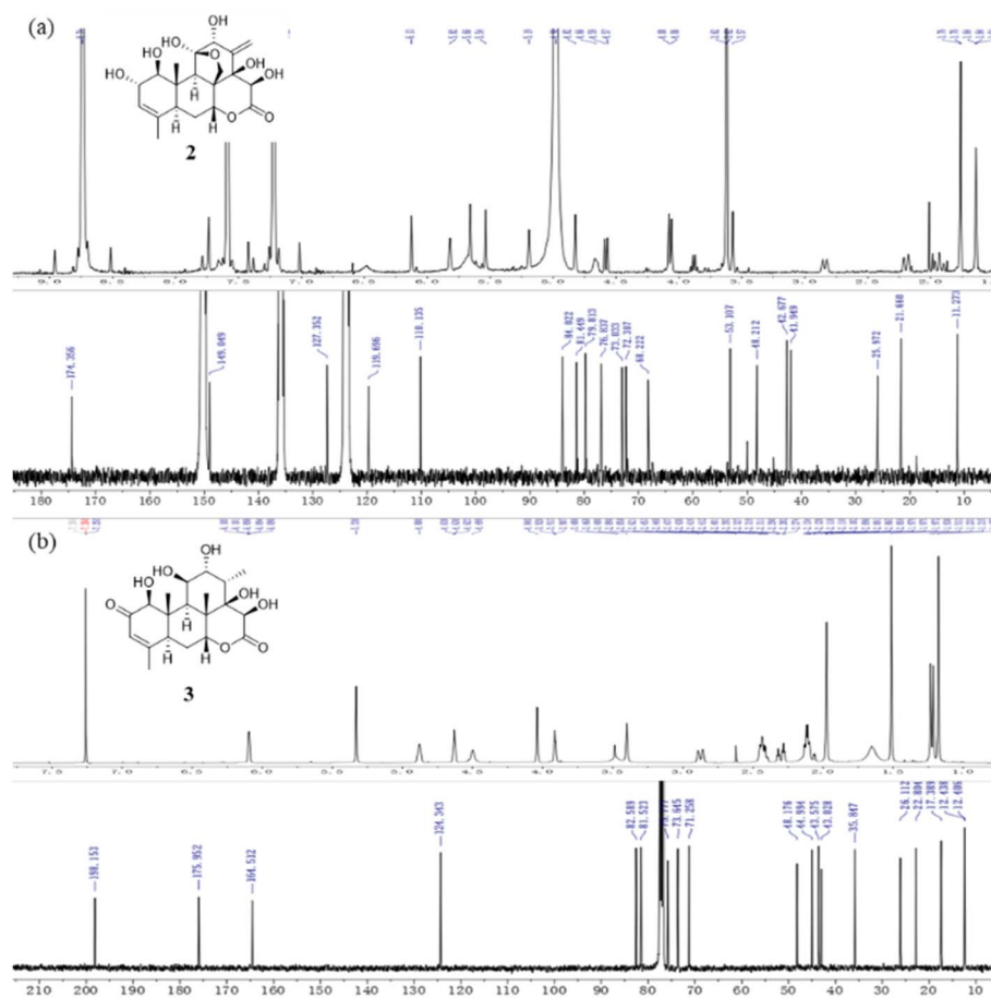
Fig. 4 (a) Eurycomanol ( 2 ): chemical structure and ^1\text{H}/^{13}\text{C} NMR spectra; (b) 14,15 \beta -dihydroxyklaineaneone ( 3 ): chemical structure and ^1\text{H}/^{13}\text{C} NMR spectra.
