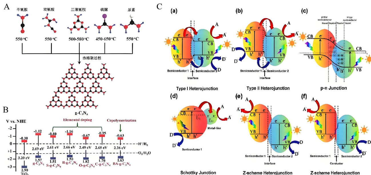
Fig. 5 Energy band structure of doped g-C 3 N 4 synthesized by thermal polycondensation. (A) g-C 3 N 4 was synthesized from several precursors by thermal polycondensations. 80 (B) Energy band diagrams of TiO 2 and g-C 3 N 4 , along with their commonly used dopant species. 80 (C) Illustrative representation of the energy band configuration of various types of heterojunctions. 81
