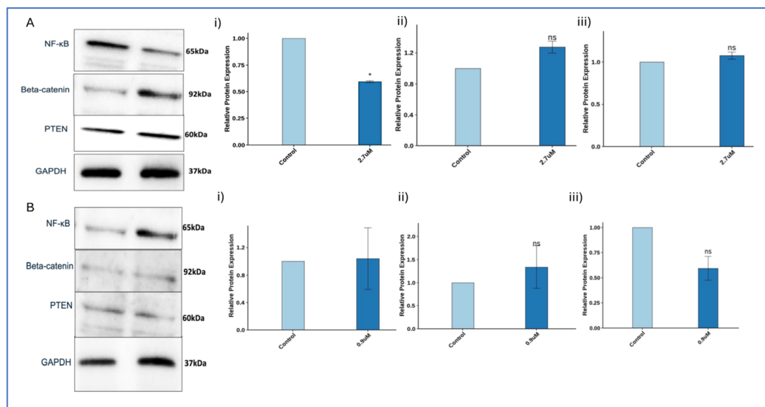
Fig. 4 GSK-3β inhibitors induced alterations in MOLT4 cells: (A) western blot analysis of GSK-3β targets 6Eb (GSKi) (A) treated MOLT4 cells lysates and 6Ec (B) and corresponding quantitation (i, ii, iii) of NF-κB, β-catenin and PTEN. Each experiment was done in duplicates, and a representative image is shown for each marker. Quantification was done for each marker (i, ii, iii) and is represented as a bar graph of mean ± SEM. One sample t -test and one way ANOVA test was performed, and the p -value were calculated between control, and compounds treated groups (*: p -value < 0.05).
