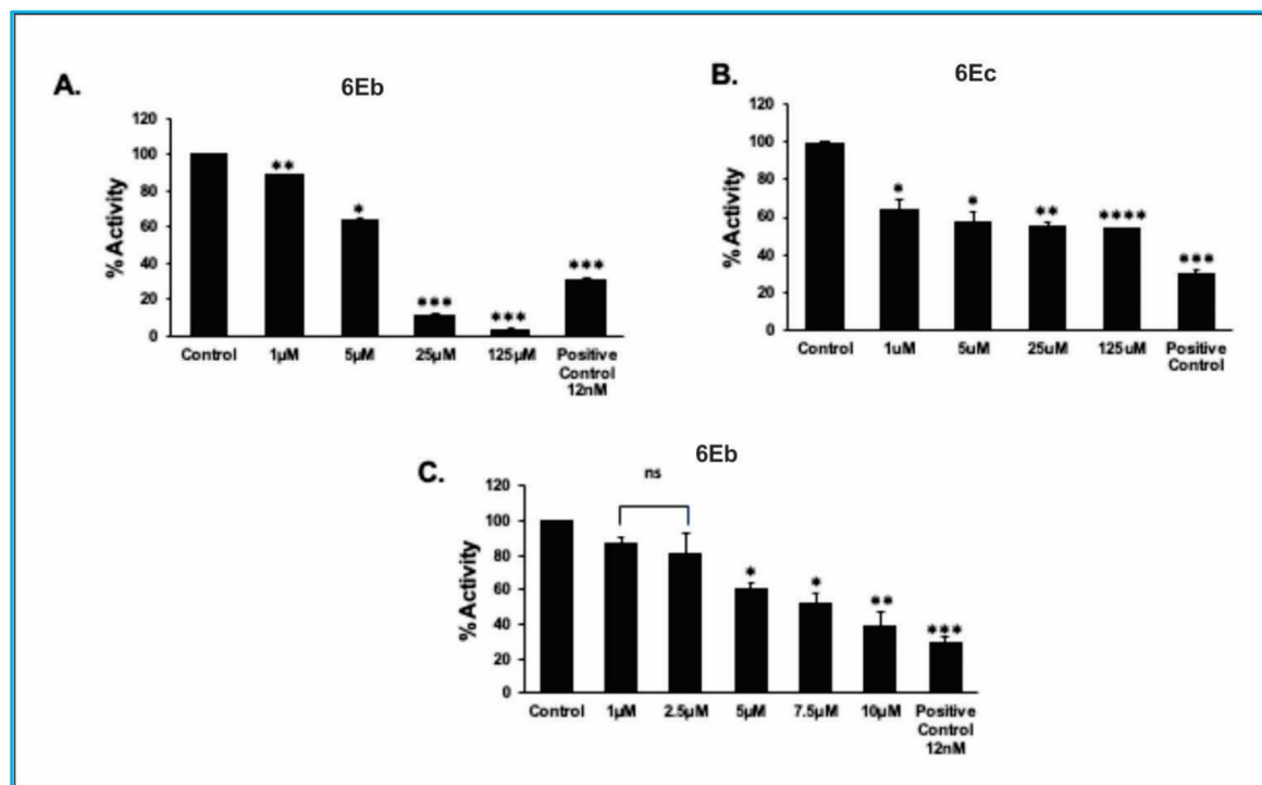
Fig. 3 The figure illustrates the dose–response relationship of compounds 6Eb and 6Ec in inhibiting GSK-3β activity. (A) Effect of compound 6Eb , at a broad range assay. (B) Effects of compound 6Ec , at a broad range. (C) Effect of compound 6Eb , at a narrower range. Data are presented as mean ± SDM. Significance was plotted based on p values and denoted as * ( p -value ≤ 0.05), ** ( p -value ≤ 0.01), *** ( p -value ≤ 0.001), **** ( p -value ≤ 0.0001) and ns as not significant.
