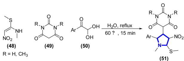
Scheme 14 Catalyst-free chemoselective synthesis of pyrrolidine derivatives.
