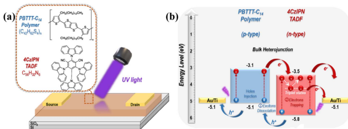
Fig. 101 (a) Diagram of the device structure and (b) energy level diagram in PBTTC-C14 polymer and 4CzIPN bulk heterojunction photo-transistor. Reproduced from ref. 305 with permission from John Wiley & Sons, Copyright © 2024, Wiley-VCH Verlag GmbH & Co. KGaA, Weinheim.
