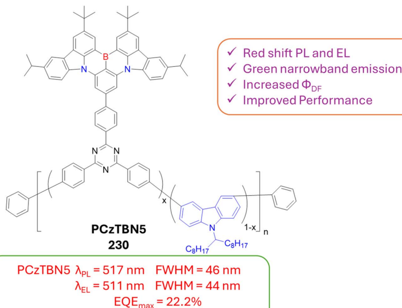
Fig. 84 Green MR-TADF and its attachment with MR emitting moiety acts as a pendant to an acceptor triphenyltriazine and simultaneously embeds acceptor moiety into polycarbazole backbone.
