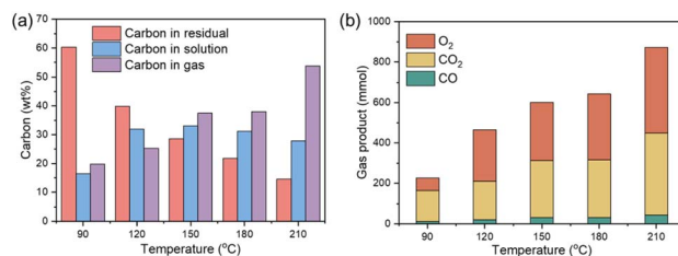
Fig. 4 (a) Distribution of carbon in the gas, residual, and solution phases of the final products; (b) distribution and composition of the gas products. The reactions were conducted for 12 hours with 2.5% \text{H}_2\text{O}_2 at varying temperatures (90–210 °C).
