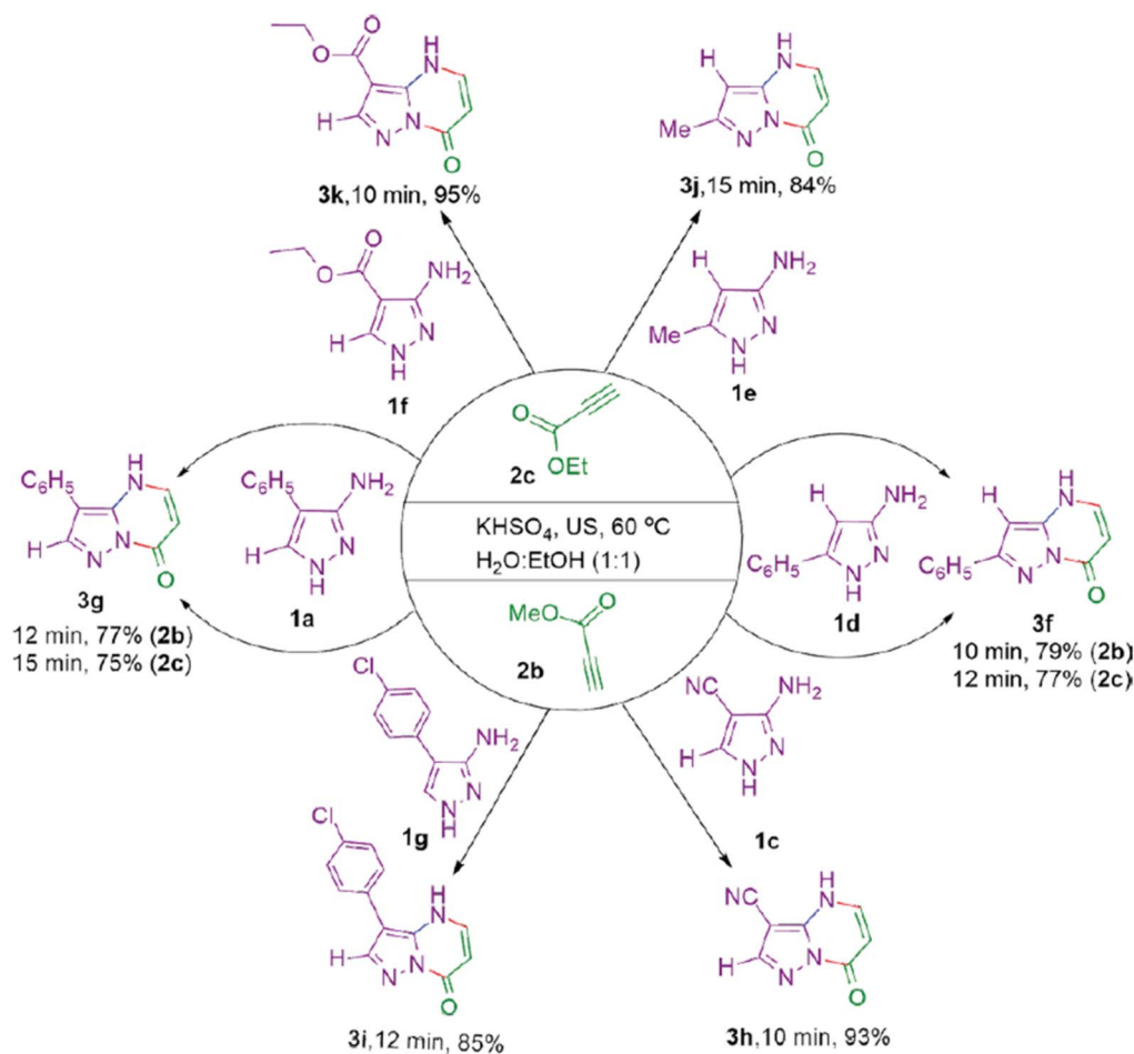
Scheme 21 Synthesis of a 2 or/and 3-substituted pyrazolo[1,5- a ]pyrimidine-7(4H)-one. 106
